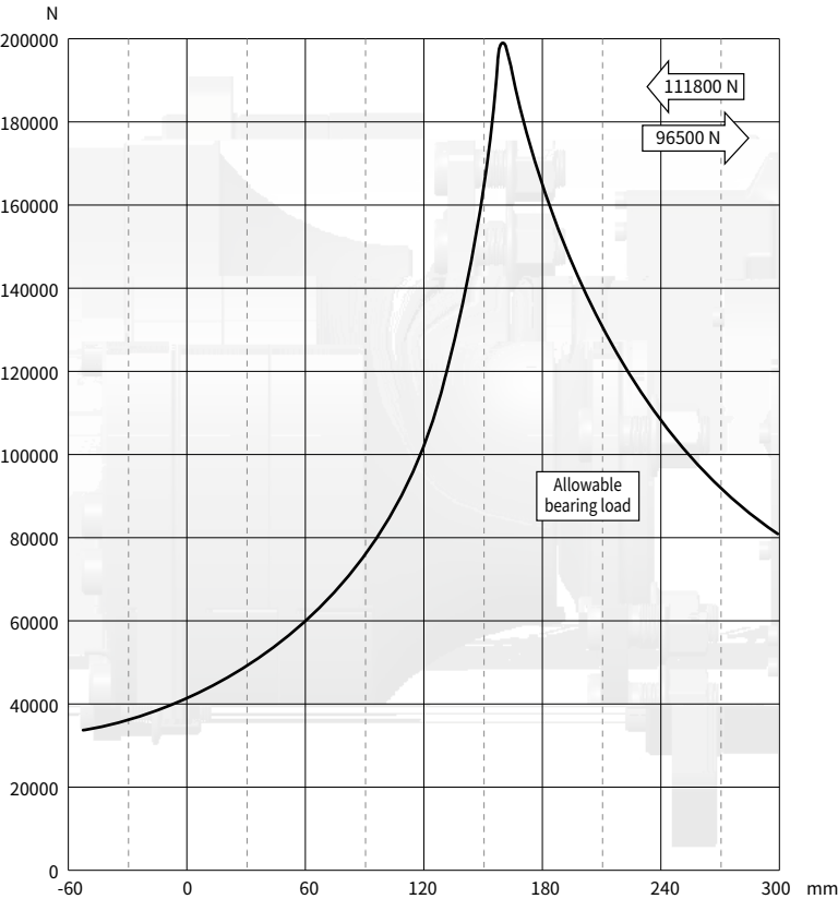
·W1/W2 Wheel Output Bearing Curve
